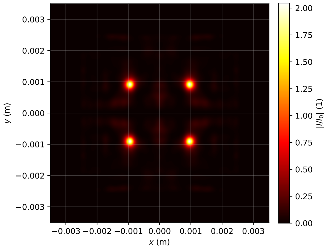
Intensity profile I(x, y, z = 3.105)/I_0 , P_{in}=9.0P_{cr} , artificial time
